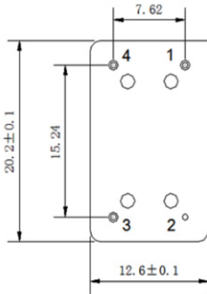
Bottom View
