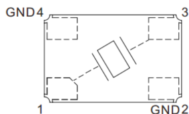
Top View Crystal Connection
