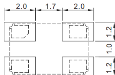
Top View Suggested Layout
