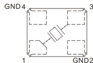
Top View Crystal Connection
