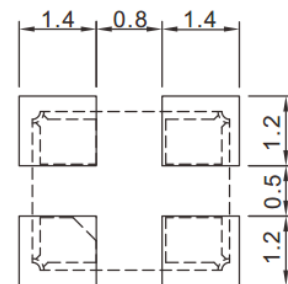
Top View Suggested Layout
